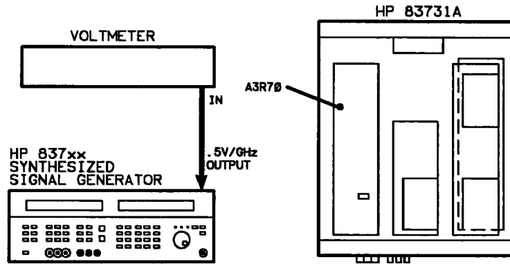
Figure 6-4. 0.5 V/GHz Output Equipment Setup
